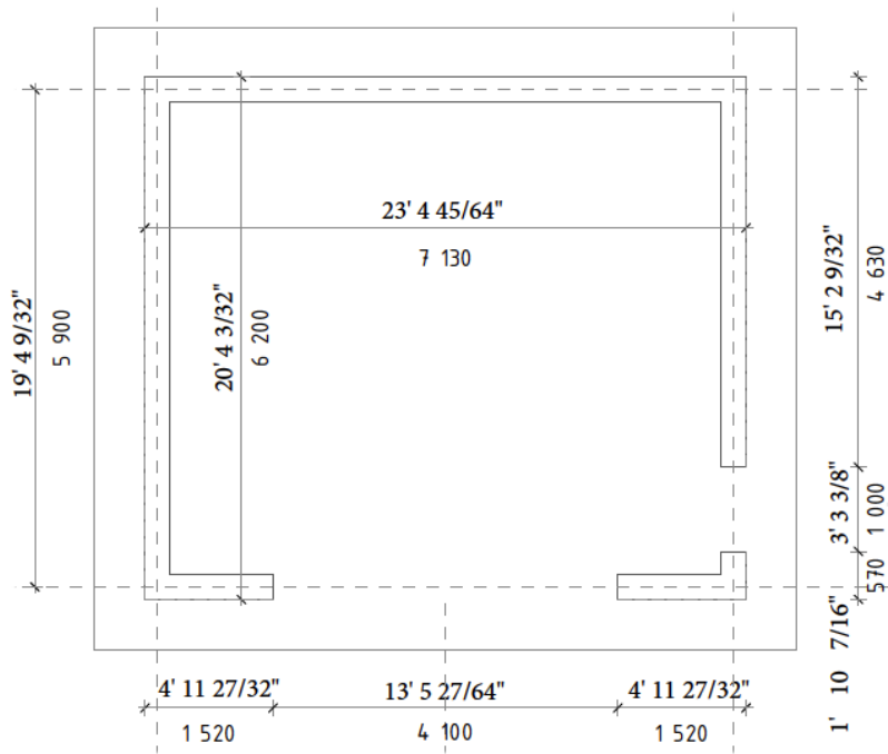
Foundation plan, Scale 1:50
