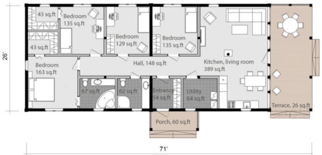
FLOOR PLAN OPTION #2
