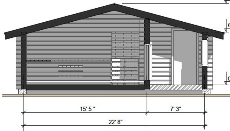
Section 1-2
