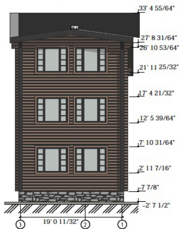
Elevations 3-1
