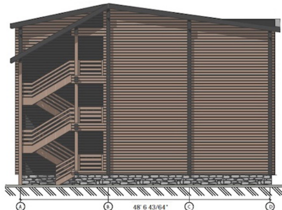
Elevations A-D
