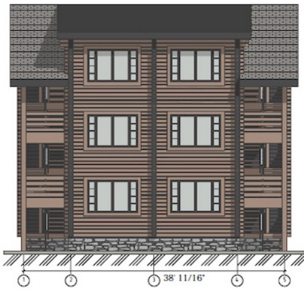
2 Sections
