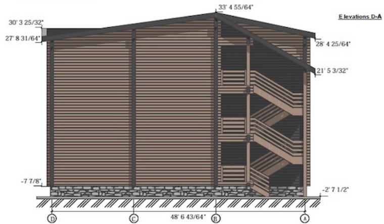
Elevations
