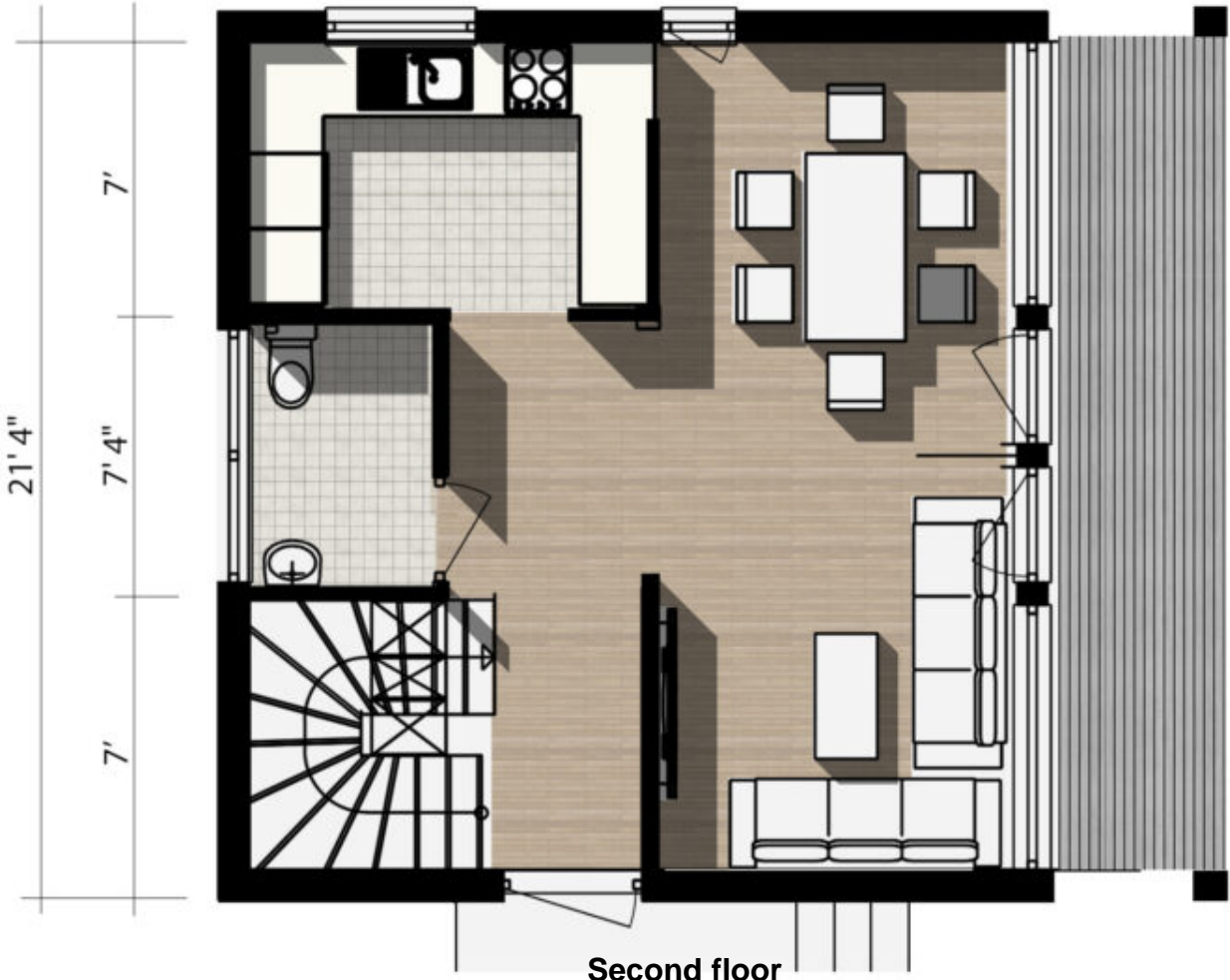
Second floor
