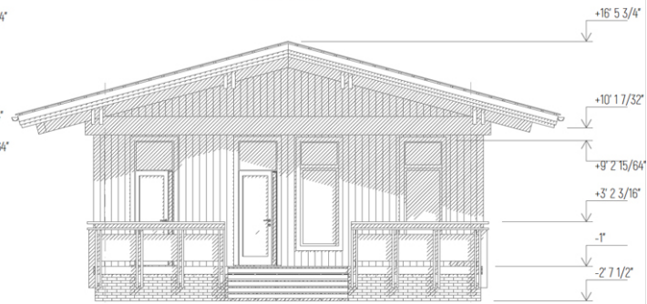
Elevation 5-1
