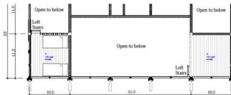
Loft floor plan
